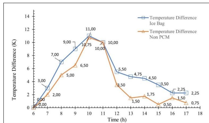
Figure 8. Temperature difference
