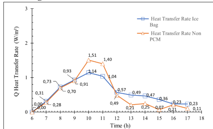
Figure 9. Heat transfer Rate
