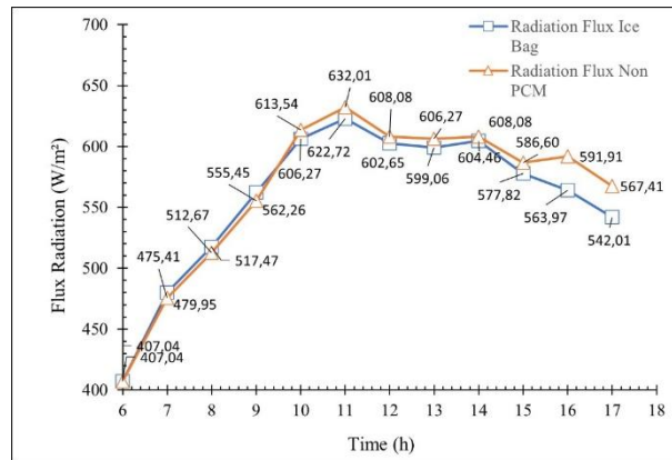
Figure 10. Flux radiation
