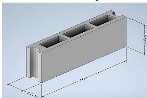
Figure 1. sketch Bricks
