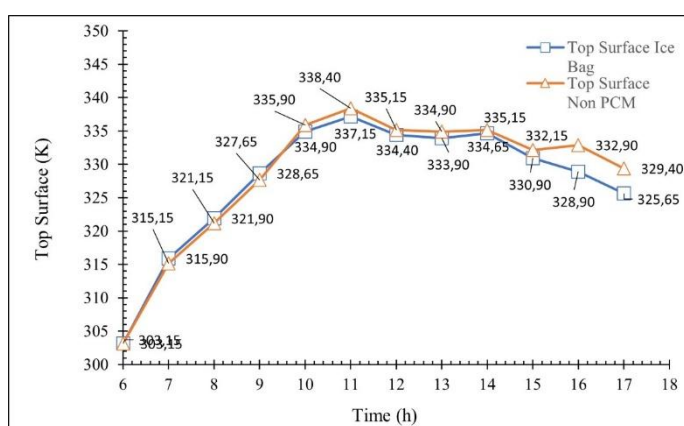
Figure 11. Top temperature surface
