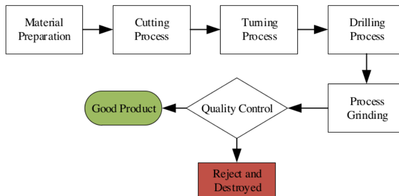
Figure 1. Flowchart Making process Dowel Pin
