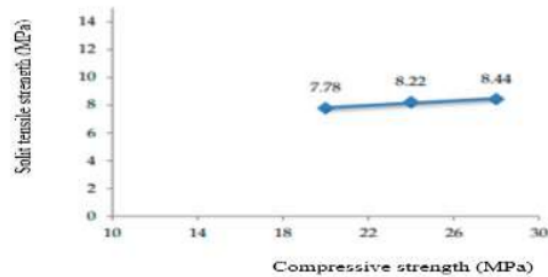
Figure 4.4. Relationship of Tensile Strength to Compressive Strength of Plan
