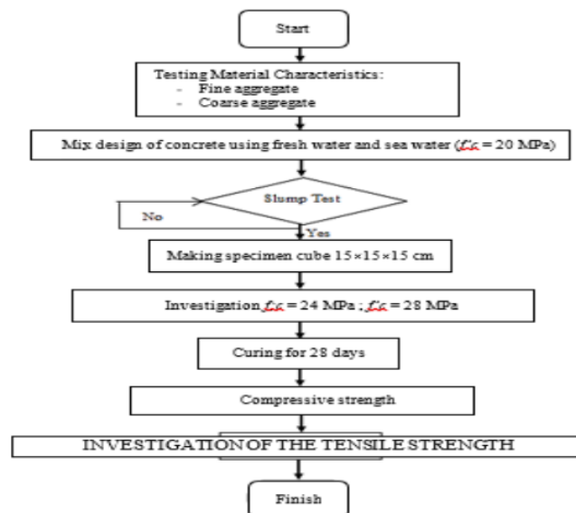
Figure 3.1. Flow chart
