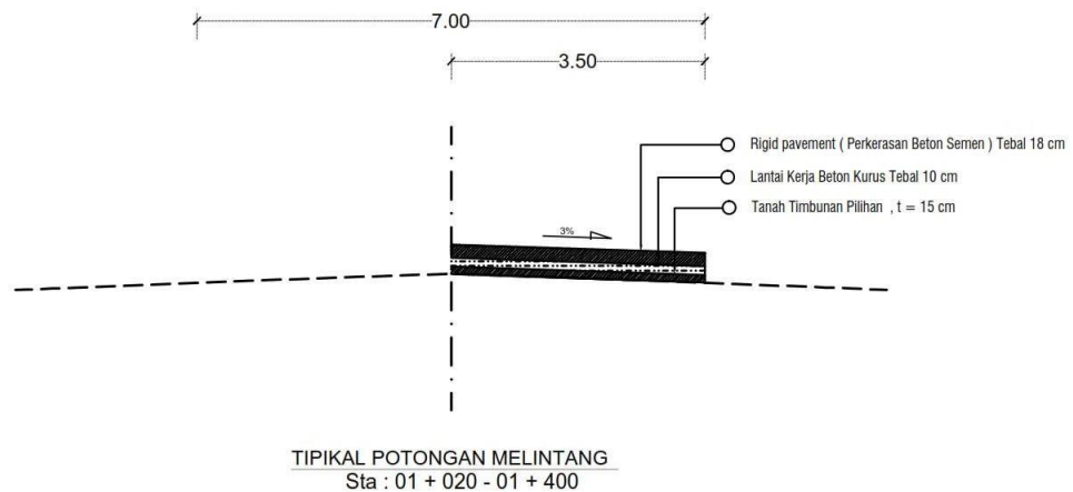
Picture 4.2 Thick Pavement Rigid Pavement According to Method Binamarga Pd T-14-2003
