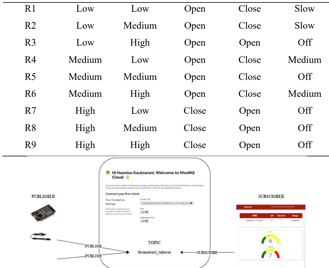
Figure 4 Schematic Diagram of MQTT Implementation
