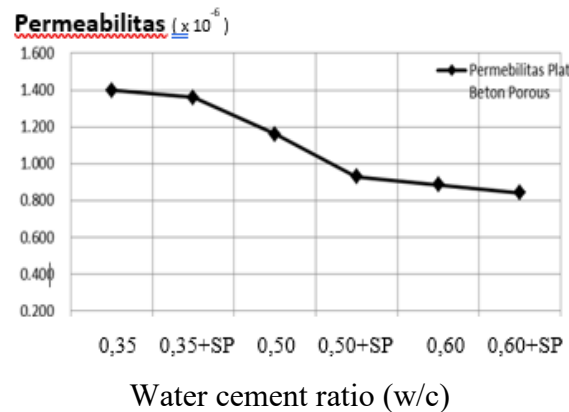
Figure 4.5 Diagram of the relationship between water-cement ratio and permeability
