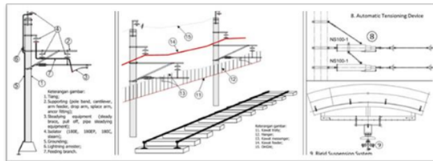
Figure 2. Overhead Contact System in MRTJ
