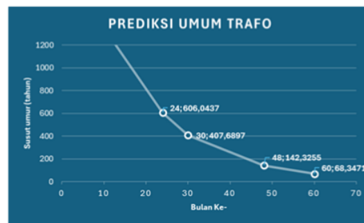
Figure 5. Graphic of Predicted Aging of Traction Transformer 1
